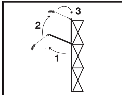
Rotate top section of strut up and slide down onto top stud.
