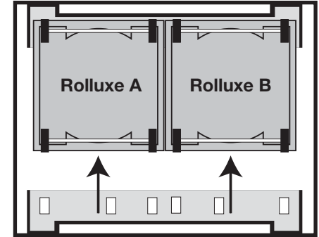
Place second wheel stop on the floor under the opposite wheels.
