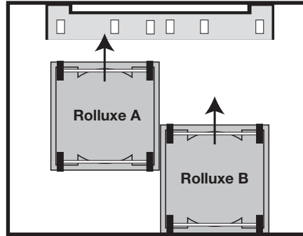
Place one wheel stop on the floor and roll the cases on to it.
